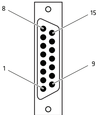
15-Pin D-sub Male
