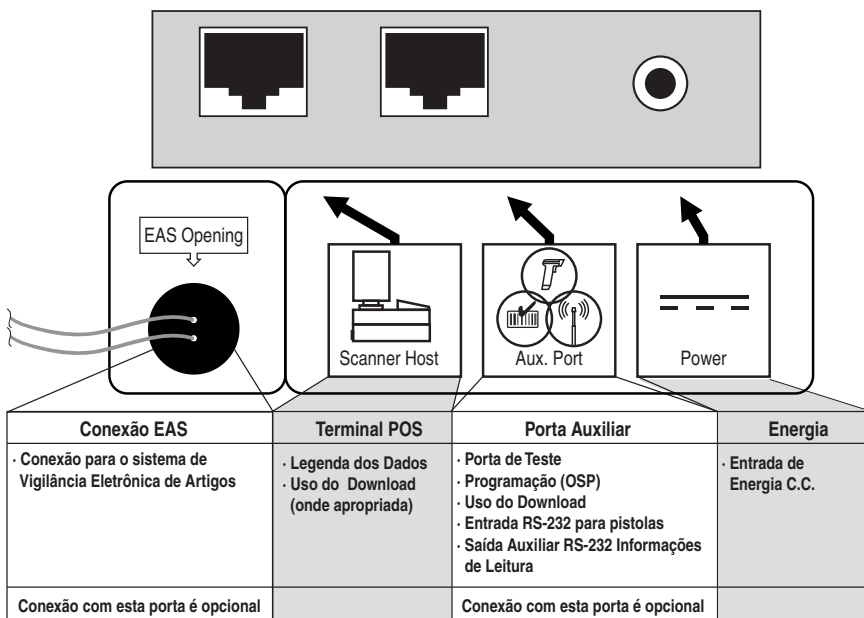
Figure 11. Conexões
