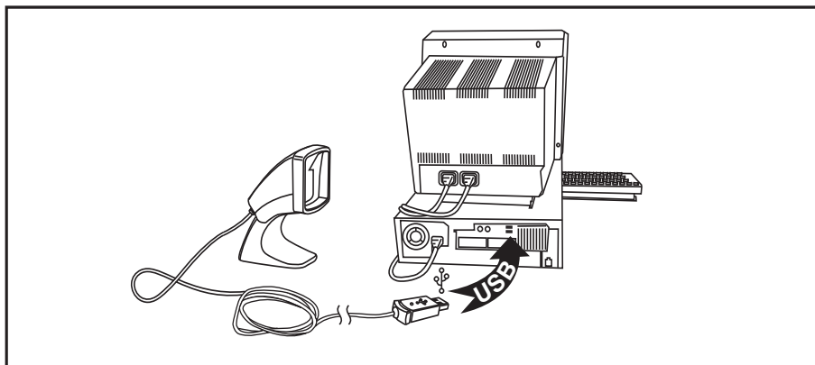
Figure 2. USB Connection
