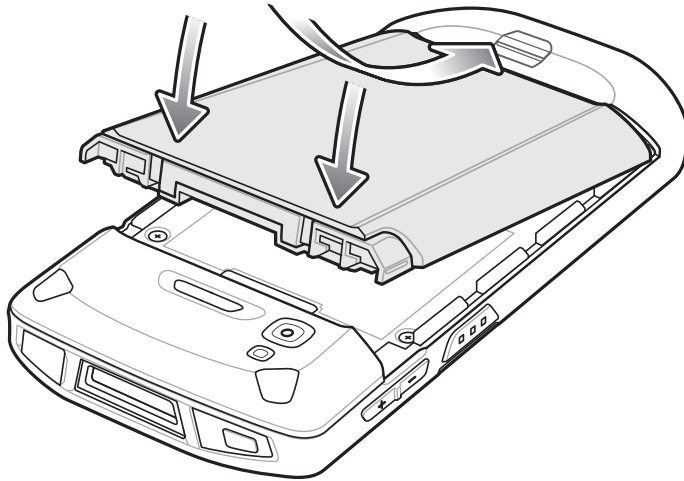
Figure 1-7 Insert Bottom of Battery into Battery Compartment
