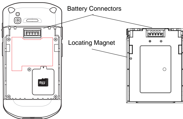
Figure 7-1 Battery Connectors and Locating Magnet
