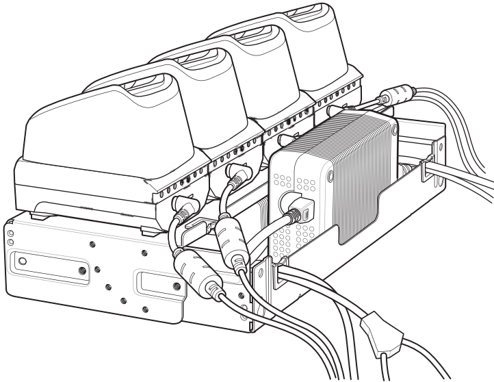
Figure 2-40 Connect Cables
