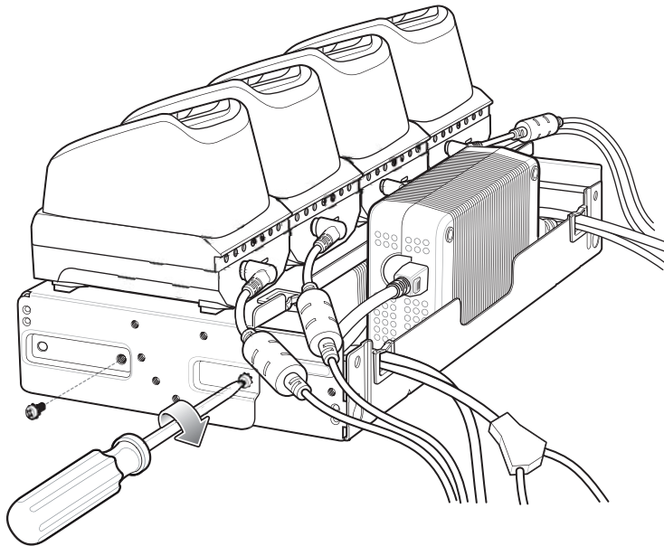
Figure 2-41 Secure Top Tray to Bottom Tray
