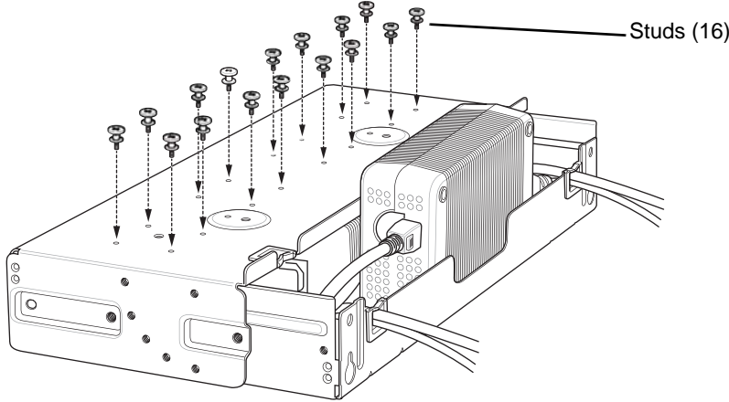
Figure 2-38 Install Studs
