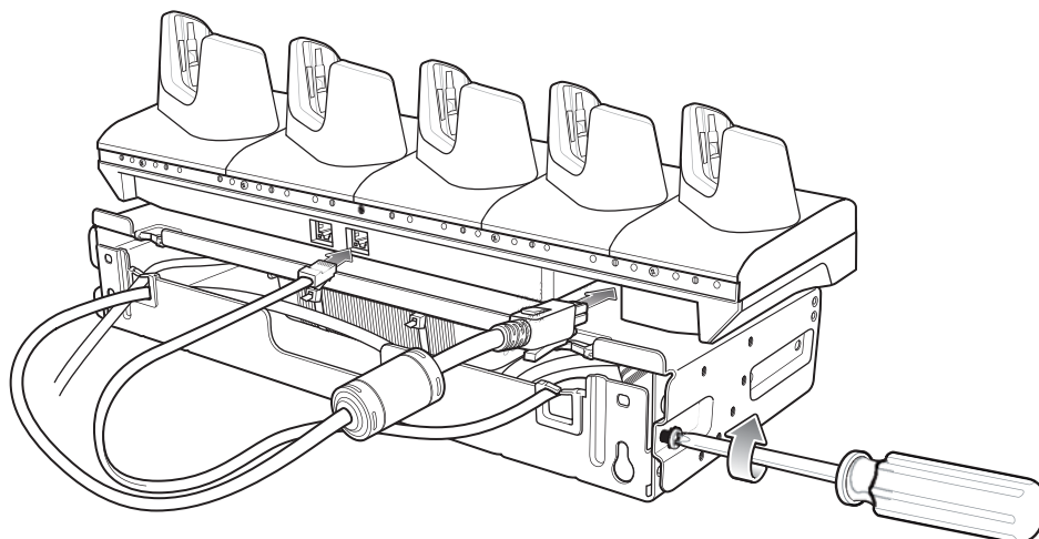
Figure 2-35 Secure Top and Bottom Tray
