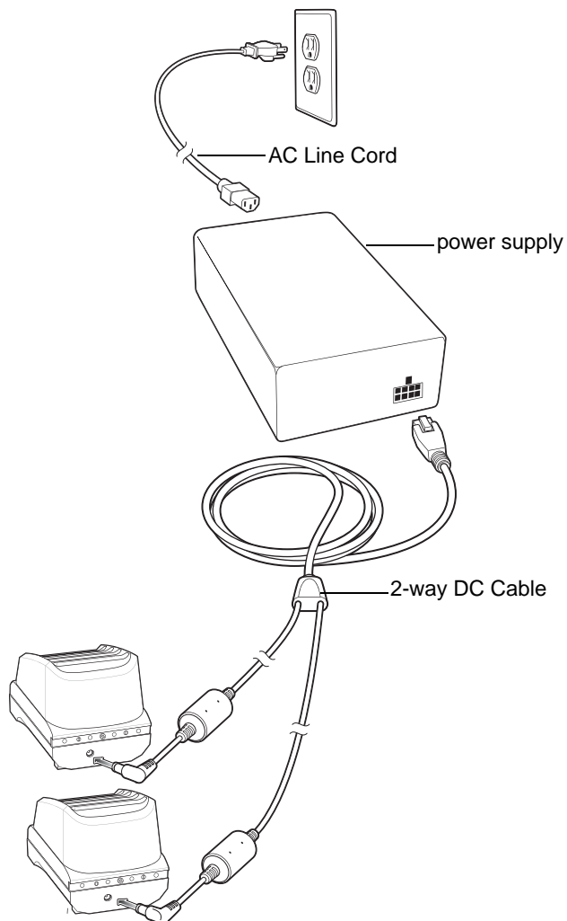
Figure 2-18 Setup with 2-Way DC Cable
