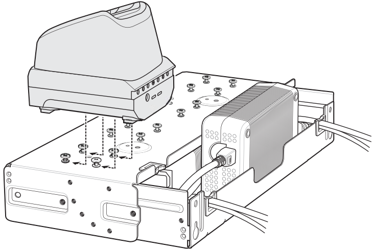
Figure 2-39 Align Chargers on Studs
