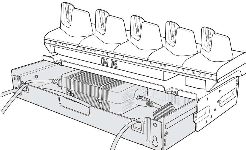
Figure 2-33 Slide Top Tray onto Bottom Tray
