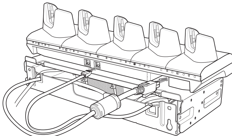
Figure 2-34 Connect Cables
