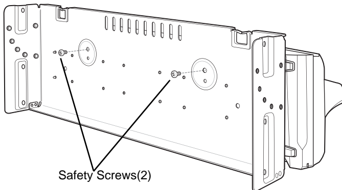
Figure 2-32 Secure Cradle
