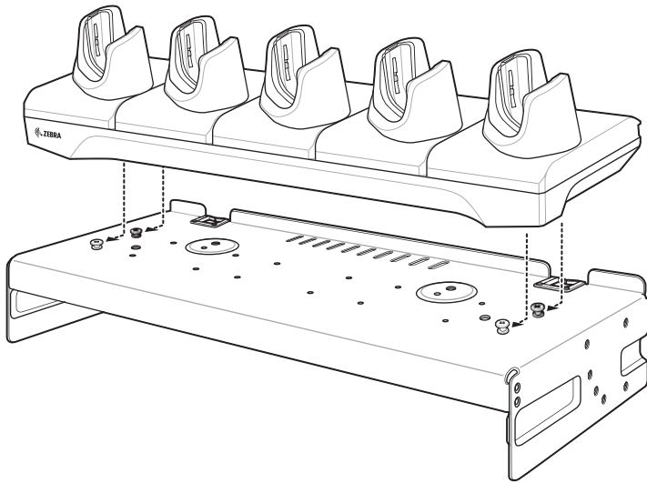
Figure 2-31 Align Cradle on Studs
