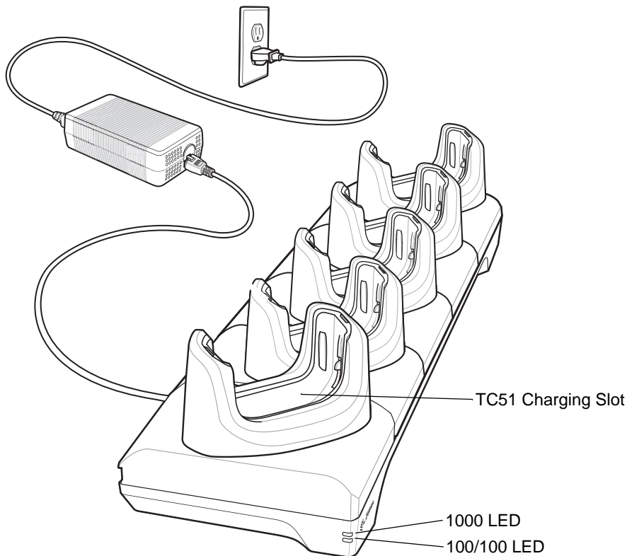
Figure 2-11 5-Slot Ethernet Cradle Setup
