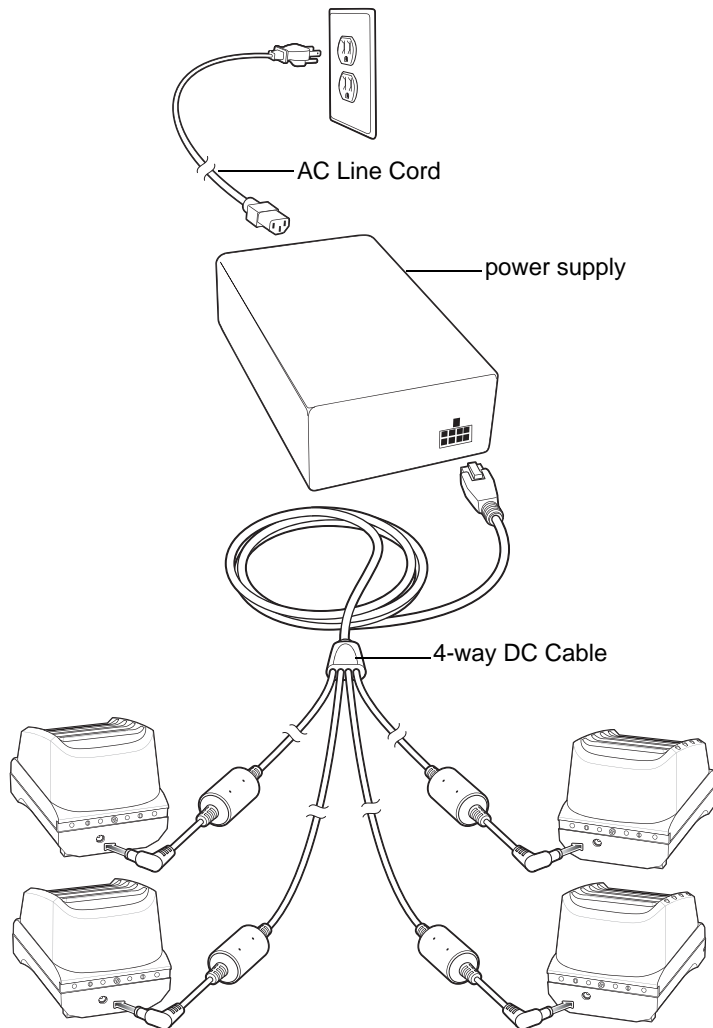
Figure 2-19 Setup with 4-Way DC Cable
