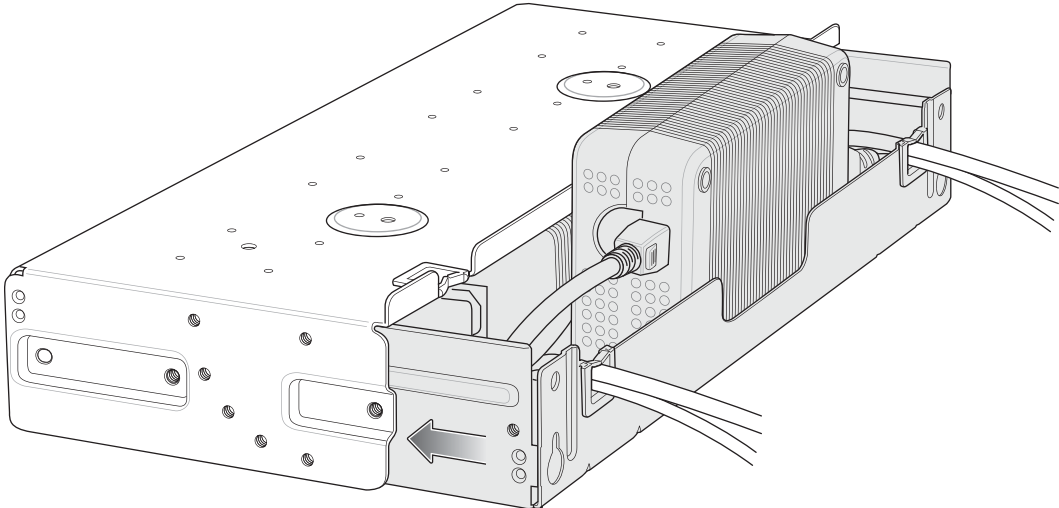
Figure 2-37 Slide top Tray onto Bottom Tray
