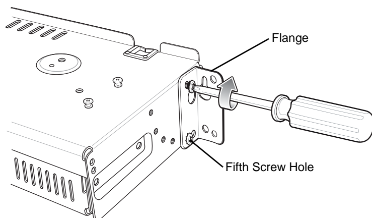
Figure 2-42 Flange Horizontal Position (5-Slot Cradles)
