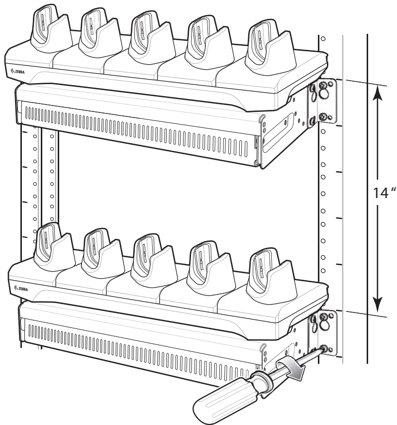
Figure 2-45 Secure Bracket to Rack (Horizontal Position Shown)
