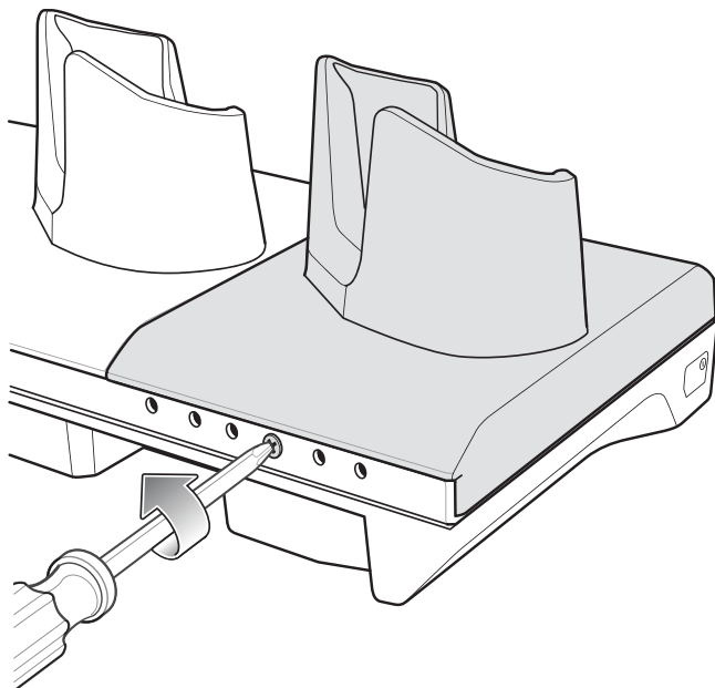
Figure 2-18 Remove Screw
