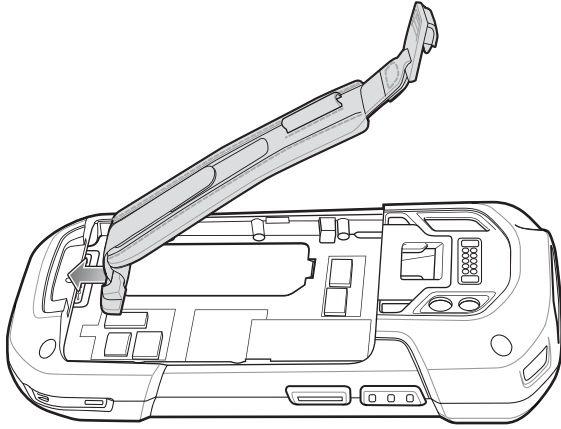
Figure 2-49 Insert Hand Strap
