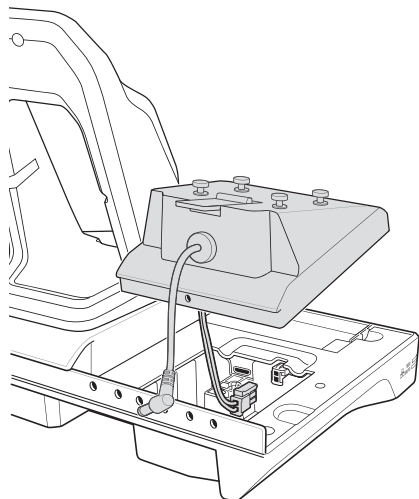
Figure 2-38 Connect Adapter Power Cable
