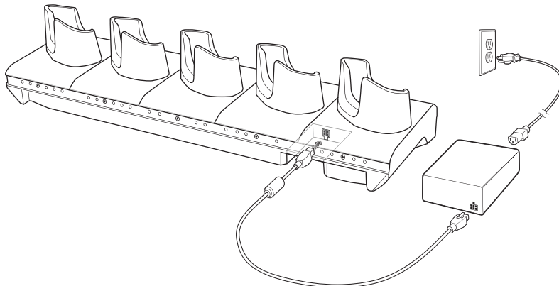
Figure 2-14 5-Slot Charge Only Cradle
