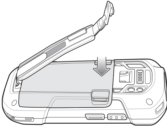
Figure 1-5 Press Down on Battery
