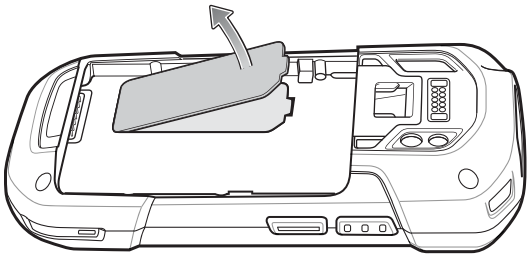
Figure 1-13 Remove Access Door
