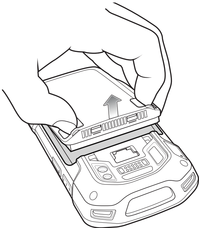
Figure 1-11 Lift the Battery
