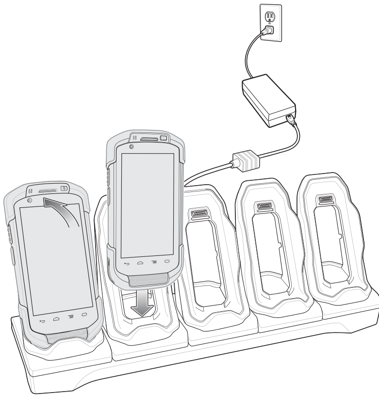
Figure 2-32 TC70 Battery Charging
