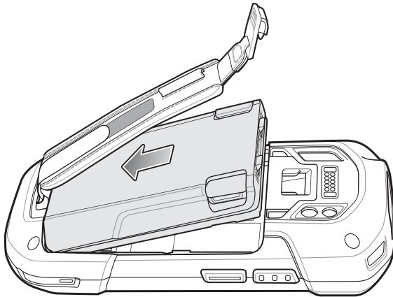
Figure 2-50 Insert Bottom of Battery into Battery Compartment
