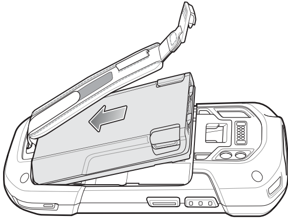
Figure 1-4 Insert Bottom of Battery into Battery Compartment
