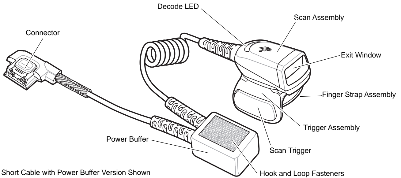
Figure 1-8 RS5000 Imager
