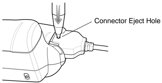
Figure 5-8 Disconnecting Connector with Shroud
