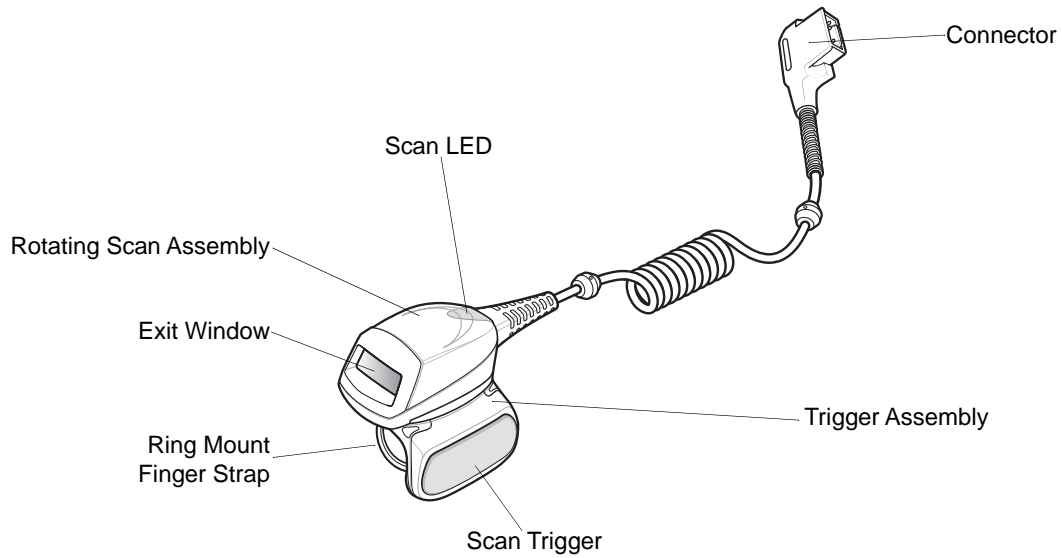
Figure 1-5 RS419 Scanner
