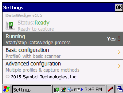
Figure 3-3 DataWedge Running
