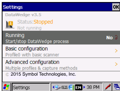
Figure 3-2 DataWedge Stopped
