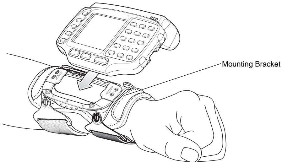
Figure 1-12 Aligning the Cleat
