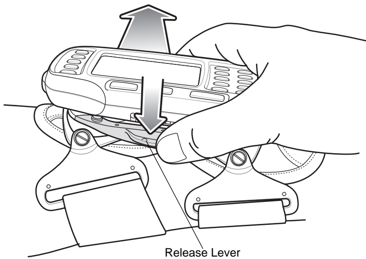
Figure 1-14 Wearable Terminal Removal
