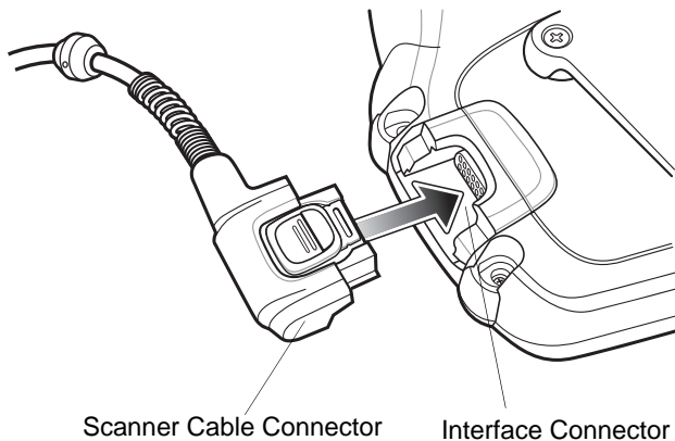
Figure 5-11 Connecting Imager to Wearable Terminal
