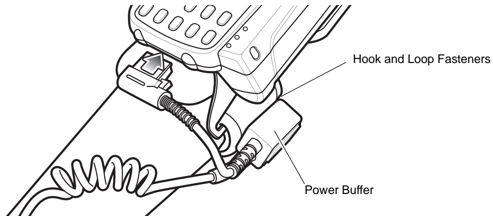
Figure 6 Attaching Power Buffer
