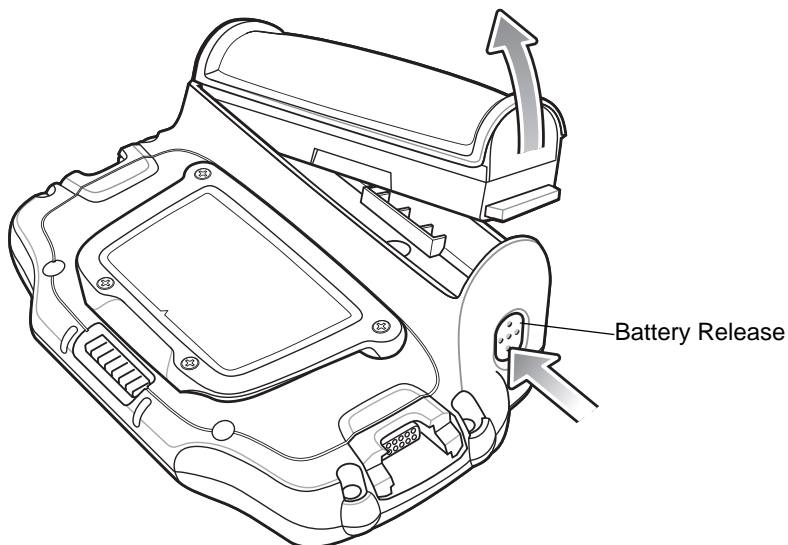
Figure 1-10 Removing the Main Battery
