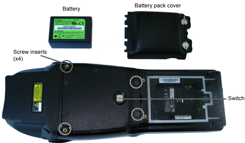
Figure 1-2 The Switch Location on the WORKABOUT PRO3
