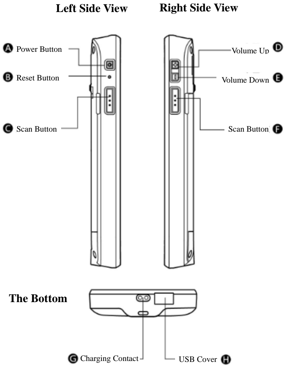
EDA50-X11 side and bottom views
