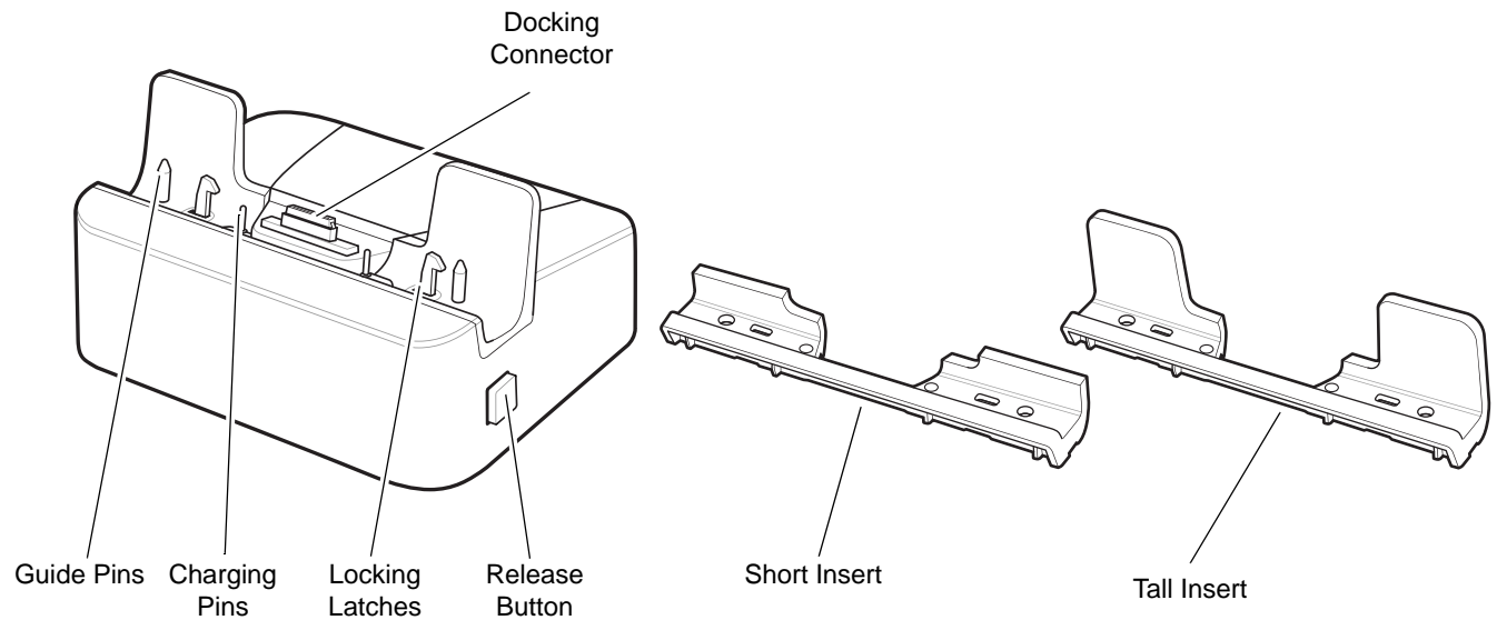
Figure 5-6 Communication and Charging Cradle - Front View
