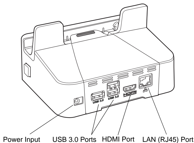
Figure 5-12 Rugged Communication and Charging Cradle - Rear View
