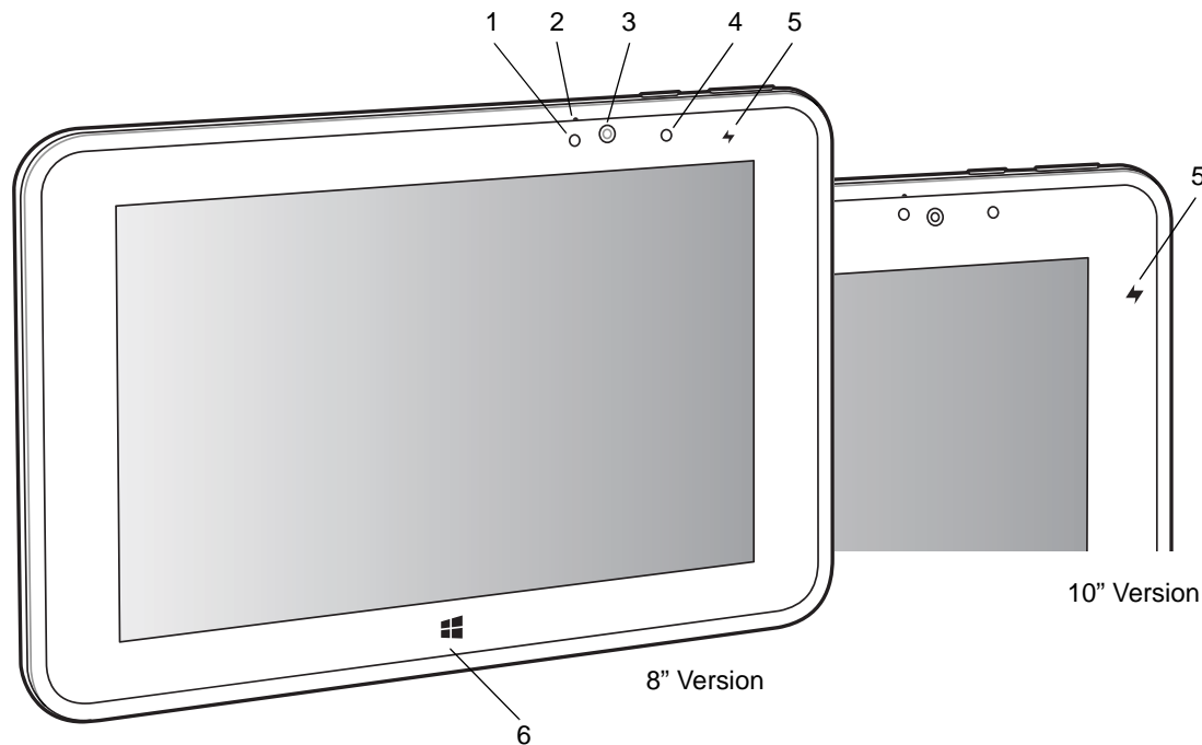
Figure 1-1 Front View
