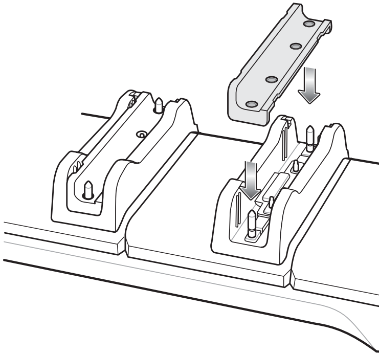
Figure 5-16 Install Insert in Slot
