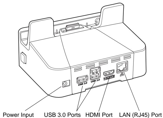
Figure 5-7 Communication and Charging Cradle - Rear View
