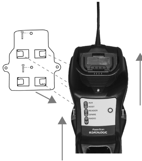
Figure 4. Mounting Plate on Wall
