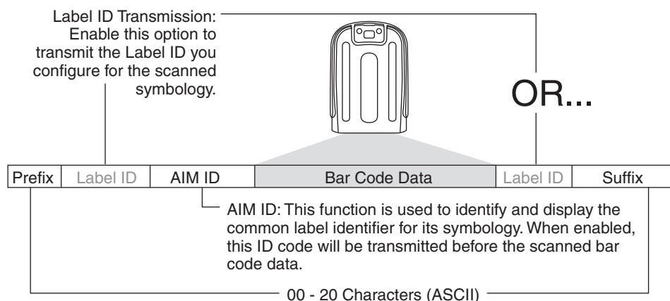
Figure 8. Breakdown of a Message String
